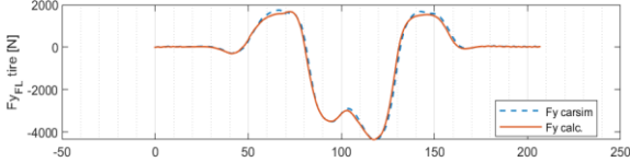
Figure 3: Lateral tire force validation of the proposed model compared to CarSim
