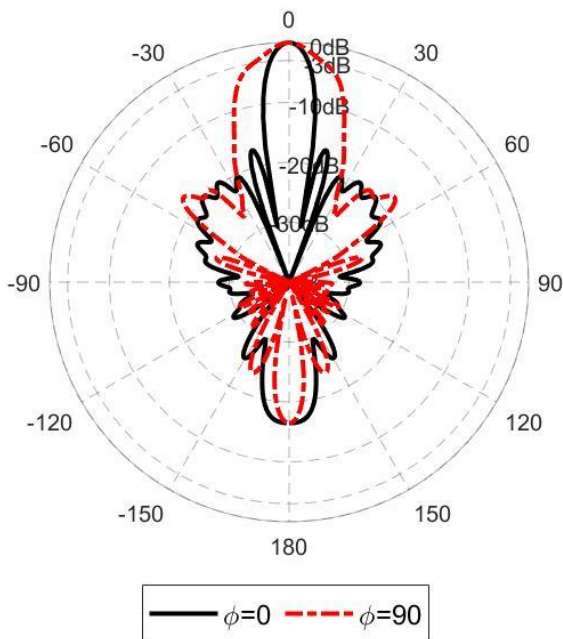
Figure 8: The polar plot of the azimuth and elevation planes
