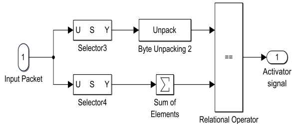
Figure 8: Checksum block
