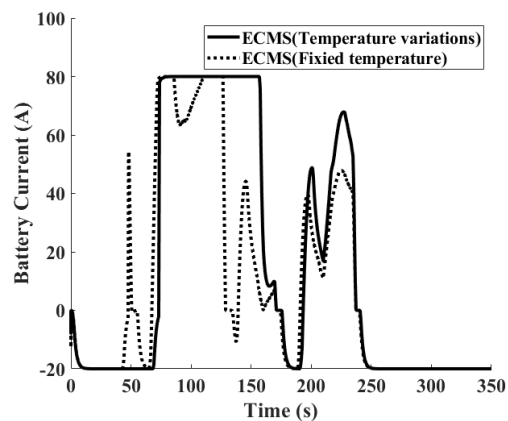
Fig.21. Battery current (comparison of both situation)
