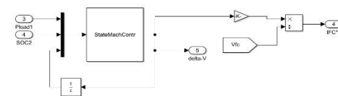
Fig.1. EMS: State machine control
