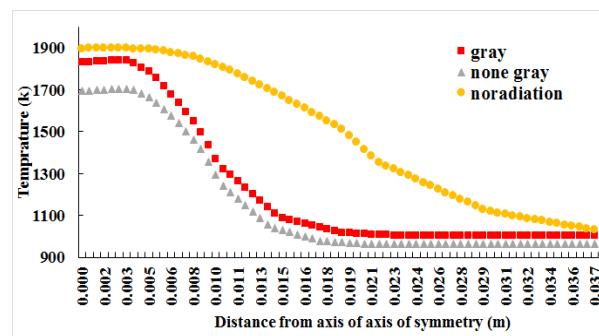
Figure 9: Radial Temperature variation
