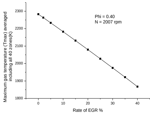
Fig6. Maximum gas temperature (Tmax) averaged including 40 zones vs rate of EGR (%)
