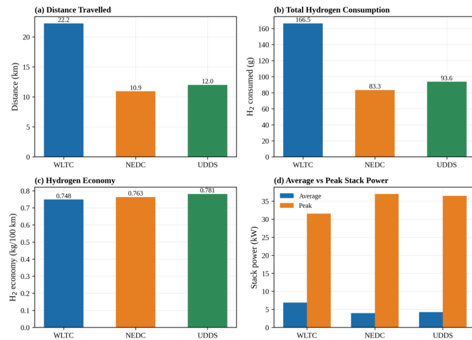
Figure 6: Comparative performance summary of the three driving cycles: (a) distance travelled, (b) total hydrogen consumption, (c) hydrogen economy, and (d) average versus peak stack power.
