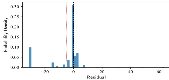
Figure 7 Distribution of residual errors for set prediction on the CHStone test set.
