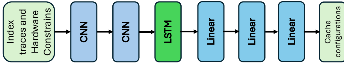
Figure 3: Model architecture
