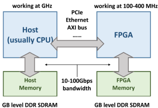
Figure 1: A typical structure of an FPGA accelerator
