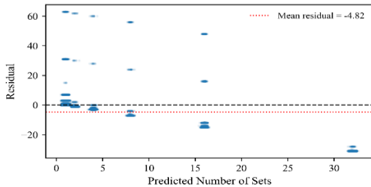
Figure 8 Residual scatter plot of set prediction errors versus predicted set values
