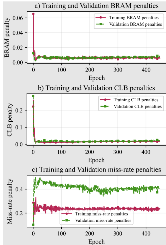
Figure 6: Transition of hardware cost and miss rate penalties throughout the training process
