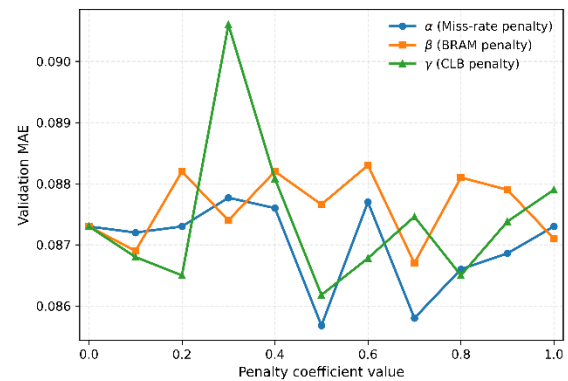
Figure 4 validation MAE obtained during first-stage one-dimensional coefficient exploration.
