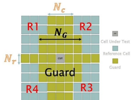
Figure 2: Windows of the proposed CFAR Algorithm
