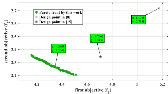
Figure 5. Pareto front as well as the design points obtained by this strategy and suggested in (Bagheri et al. 2011, Mahmoodabadi and Nejadkourki 2022).
