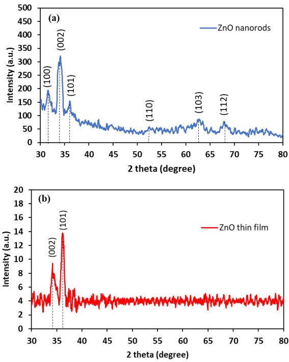
Figure 1: XRD pattern of the (a) ZnO nanorods, and (b) ZnO thin film.
