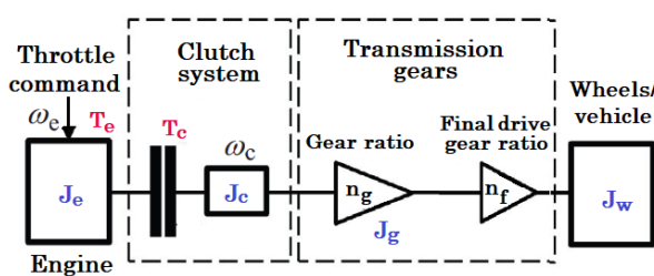
Figure 2: Simplified driveline model
