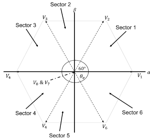
Figure 4: Sector selection of required voltage vector approach, edited from [10].
