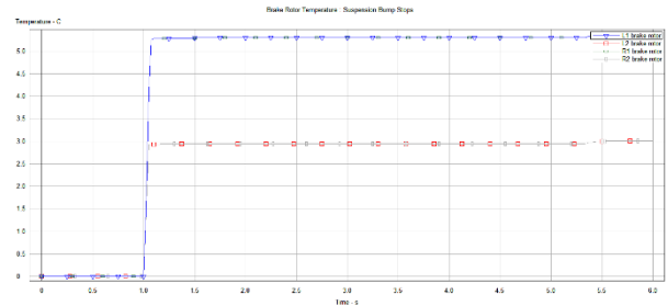
Figure 22: Brake Rotor Temperature C-Time(s) "Carsim_ABS_OFF"
