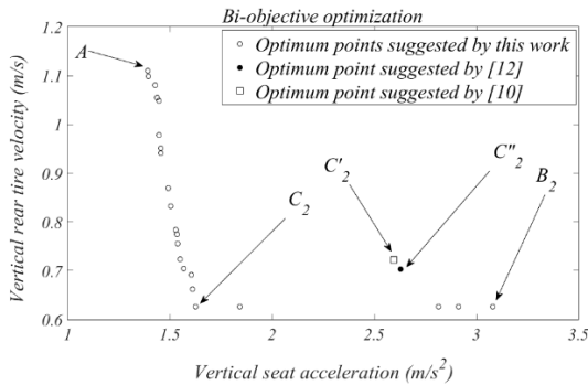
Figure 4. Pareto front of vertical seat acceleration and vertical rear tire velocity resulted by bi-objective optimization.
