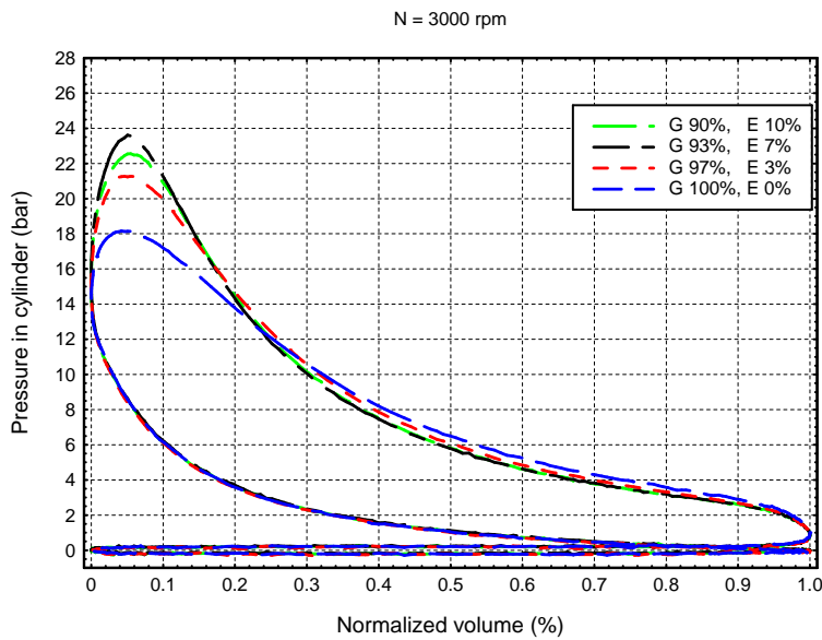
Fig.9. P-V Diagram
