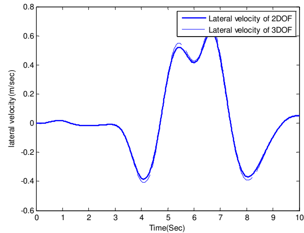
Fig6. Lateral velocity response for DLC manoeuvre
