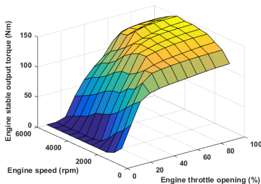
Figure 3: The EF7 engine torque map [25]
