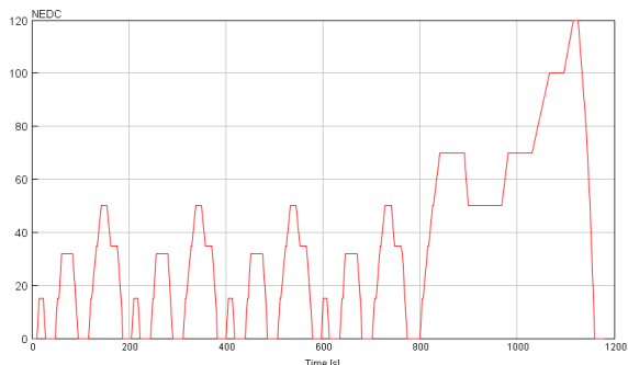
Figure 4. NEDC driving cycle
