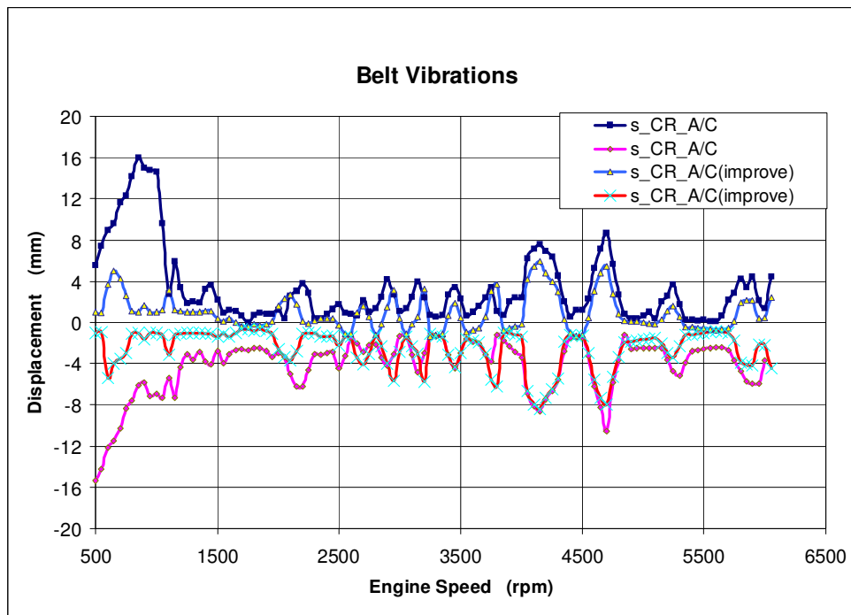
Figure 18. Belt vibration( comparison between initial layout and improve layout)
