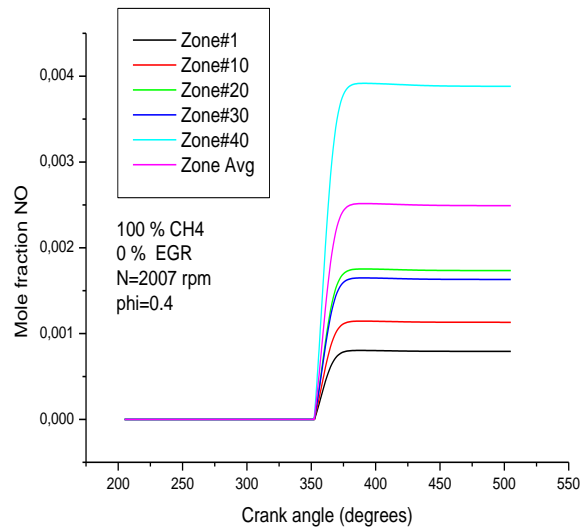
Fig10. Mole fraction of NO per CA histories (100 % CH4/0% EGR, phi = 0.40)
