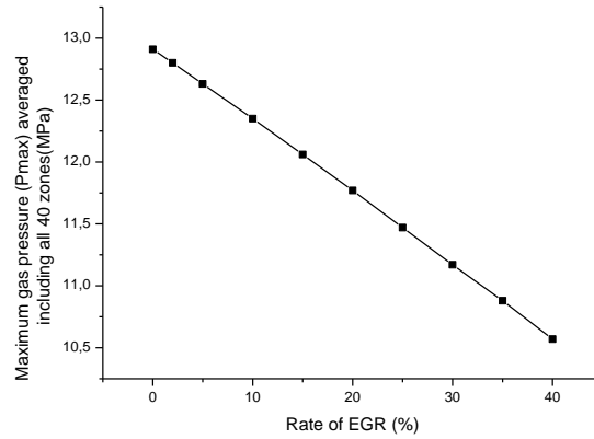
Fig5. Maximum gas pressure (Pmax) averaged including 40 zones vs rate of EGR (%)
