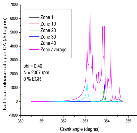
Fig7. Zone NHRR per CA histories without EGR
