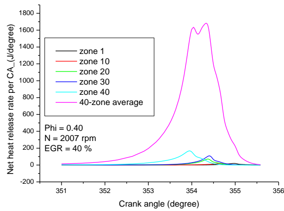
Fig9. Zone NHRR per CA histories with 40 % EGR
