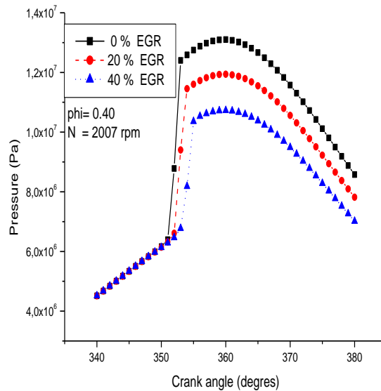
Fig1.. In cylinder pressure variation for three different EGR rate
