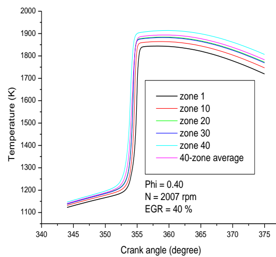
Fig4. Temperatures predicted by the multi-zone model. The energy-equation is engaged at -15.5^\circ BTDC.
