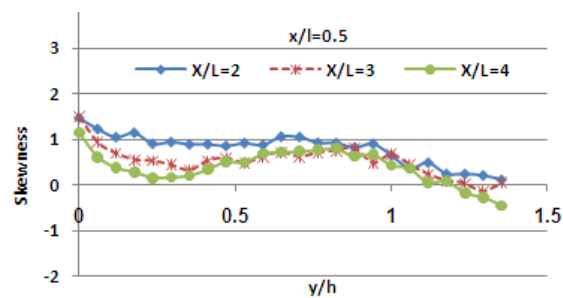
Fig5. The trend of change in skewness for different positions of car in the flat wake of the trailer for x/l=0.5
