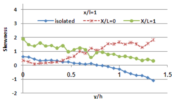
Fig6. The trend of change in skewness for different positions of car in the flat wake of the trailer for x/l=1
