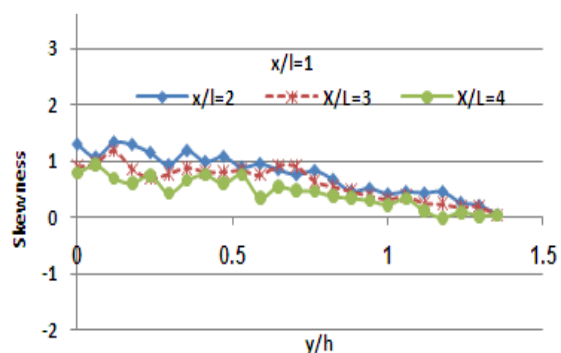
Fig6. The trend of change in skewness for different positions of car in the flat wake of the trailer for x/l=1
