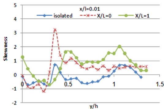
Fig4. The trend of change in skewness for different positions of car in the flat wake of the trailer for x/l=0.01
