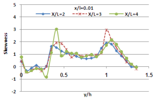
Fig4. The trend of change in skewness for different positions of car in the flat wake of the trailer for x/l=0.01
