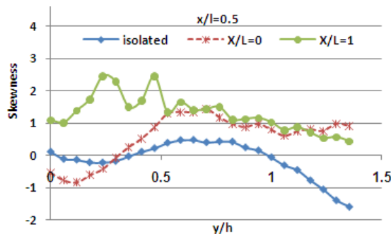
Fig5. The trend of change in skewness for different positions of car in the flat wake of the trailer for x/l=0.5
