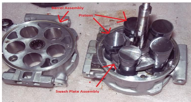
Fig.1: Five cylinder swash plate reciprocating compressor
