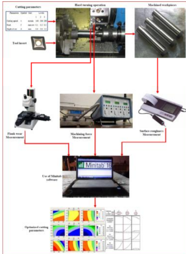
Fig1. Experimental setup
