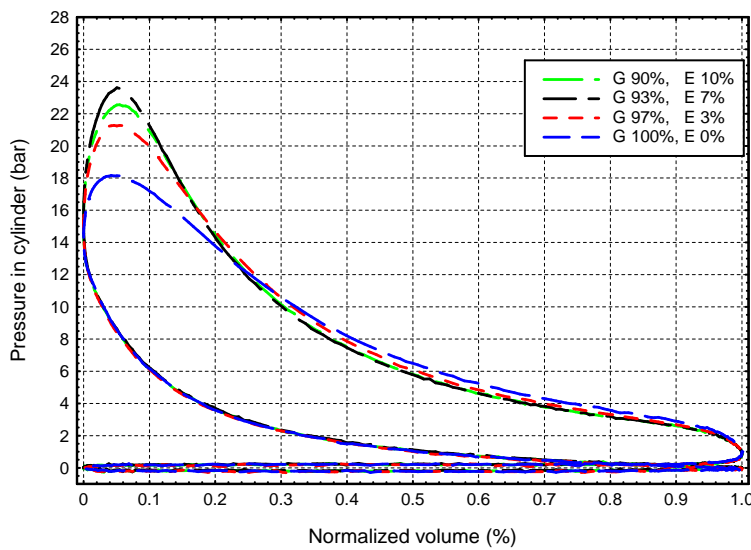
Fig.9. P-V Diagram
