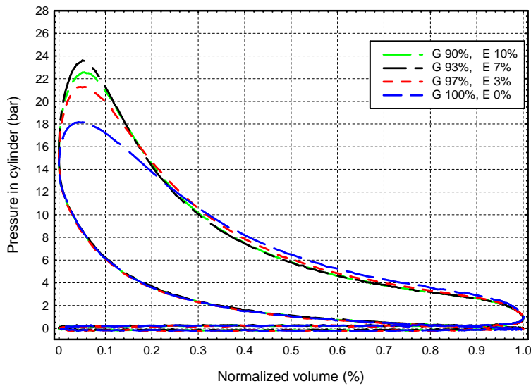
Fig.9. P-V Diagram
