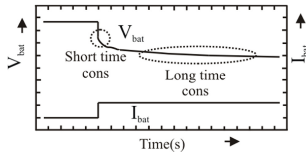
Fig2. Transient response to a step load-current
